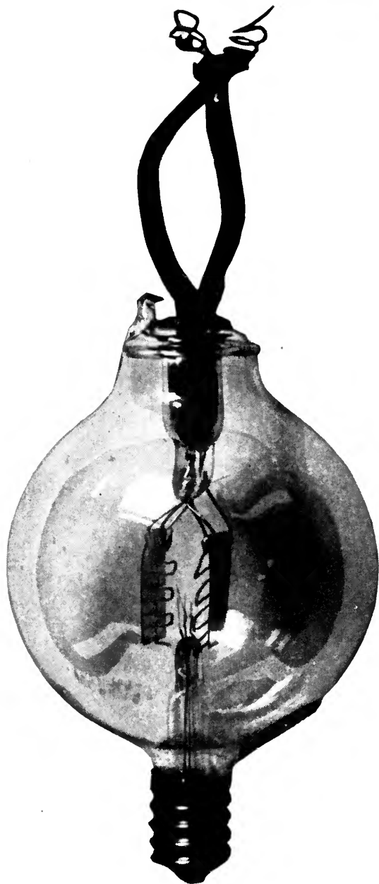
This is a real old De Forest audion. Several years ago radio amateurs saved for long periods to procure one of these magic bulbs. As may be observed, two filaments, two plates, and two grids were employed. The stability of this type tube was anything but constant due to imperfect evacuation
